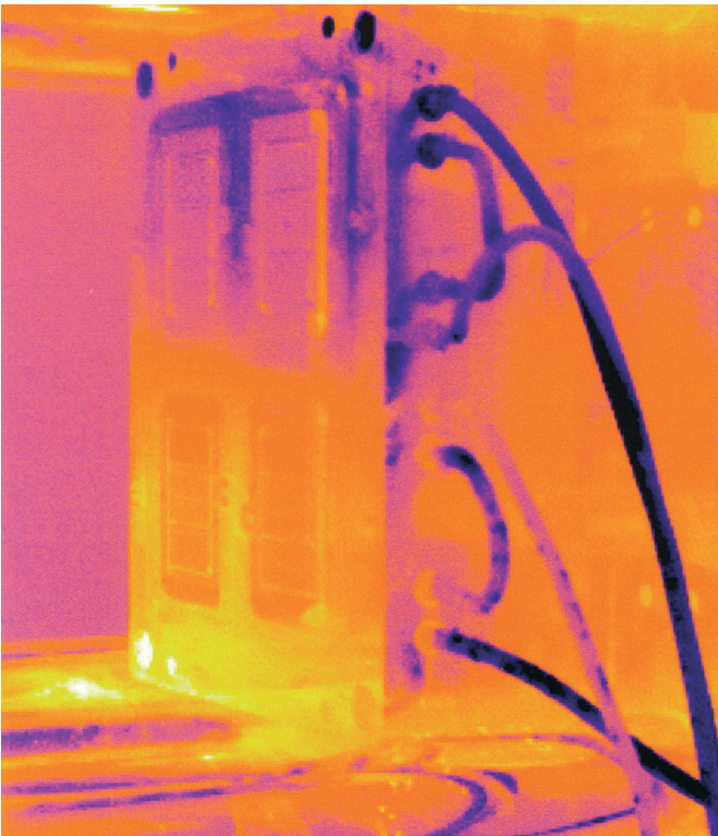
› Thermography of an injection mould Inhomogeneous increase of temperature due to the use of contaminated heating/cooling channels
